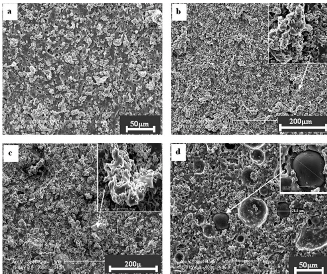
Figure 2 SEM micrographs of MR elastomers based on SR/PS with different content of PS: (a) 0%; (b) 5%; (c) 10%; and (d) 20%.
