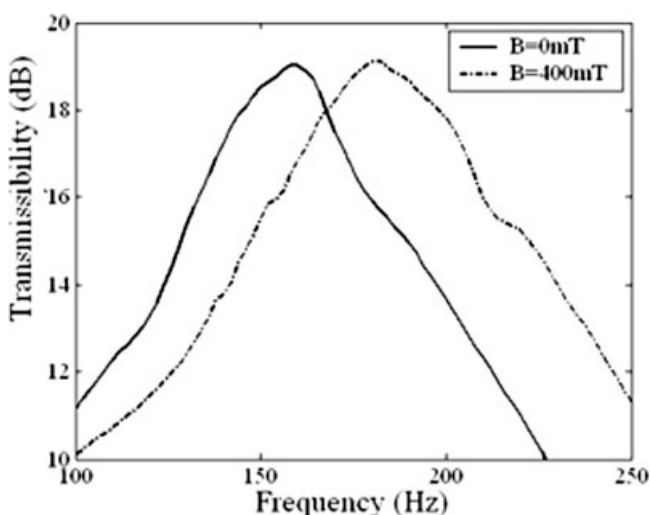
Figure 3 Frequency-dependent transmissibility of MR elastomers based on pure SR at magnetic flux density B = 0 and 400 mT.
