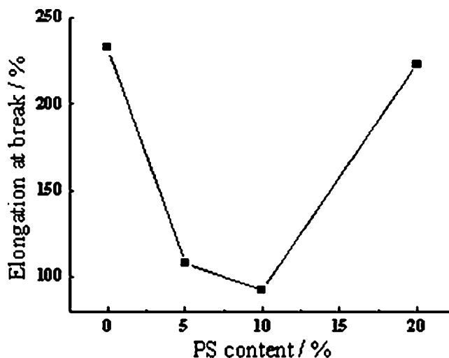
Figure 7 Effect of PS content in the SR/PS blends on elongation at break. Error < 10.
