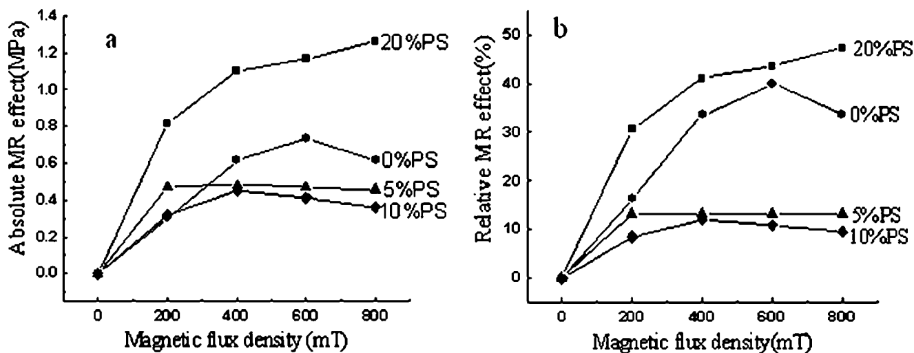
Figure 5 Absolute (a) and relative (b) MR effect as a function of the applied magnetic field for MR elastomers with different content of PS.
