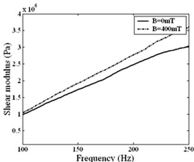
Figure 4 The shear modulus as a function of frequency at different magnetic flux fields.
