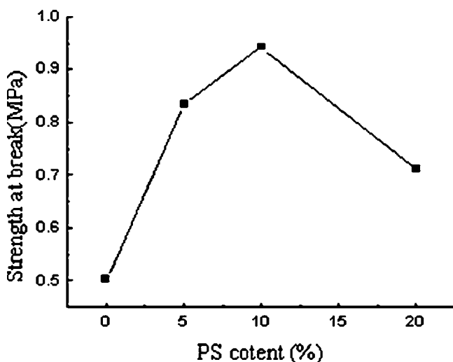
Figure 6 Dependence of tensile strength on the PS content in the MR elastomers based on SR/PS. Error < 0.05 MPa.
